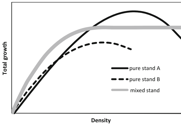
Fig. 7 Density–growth relationships in pure and mixed-species stands, modified after Pretzsch (2002). Both monospecific stands exhibit an optimum density, where total growth is maximum. The mixed stand of both species does not show an optimum density and—in this example—has a maximum growth between the two pure stands. Depending on at which density the stands are compared, the mixed stand will show transgressive overyielding (at lower densities) or not
